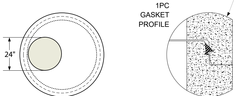
Top Cone Plan View
