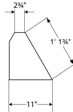
End View
