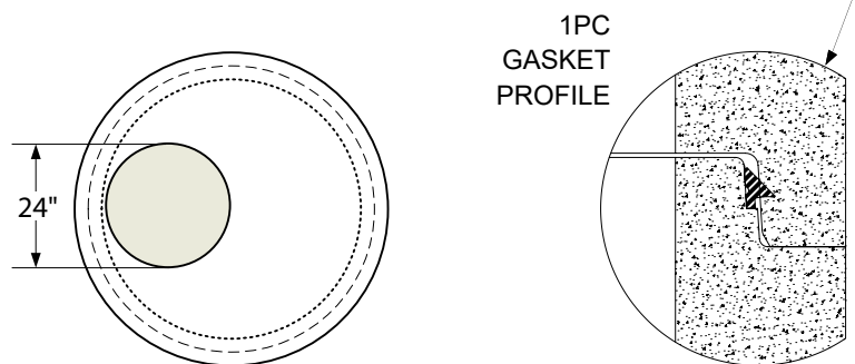
Top Cone Plan View Gasket Shown Uncompressed
